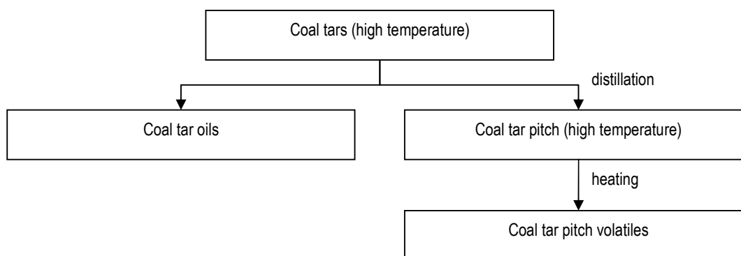
Figure 1.1.1. Origin of high temperature coal tar products.
