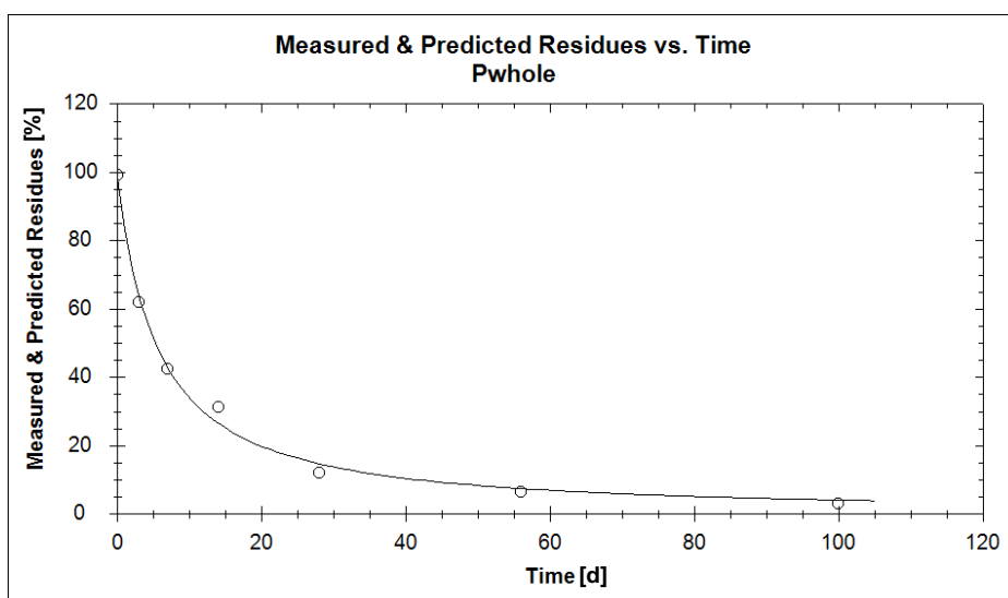
Figure 39: Measured and predicted residues of EC 407-000-3 vs. time in the whole system of an aerobic pond – FOMC.
