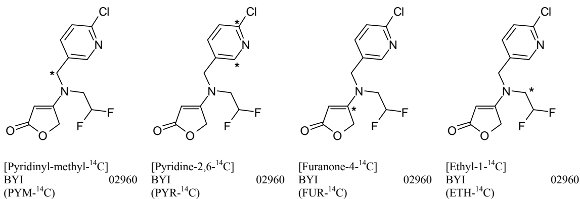
Figure 7: The structure of BYI 02960 (flupyradifurone) and the positions of the different radiolabels. * indicates position of radiolabel.
