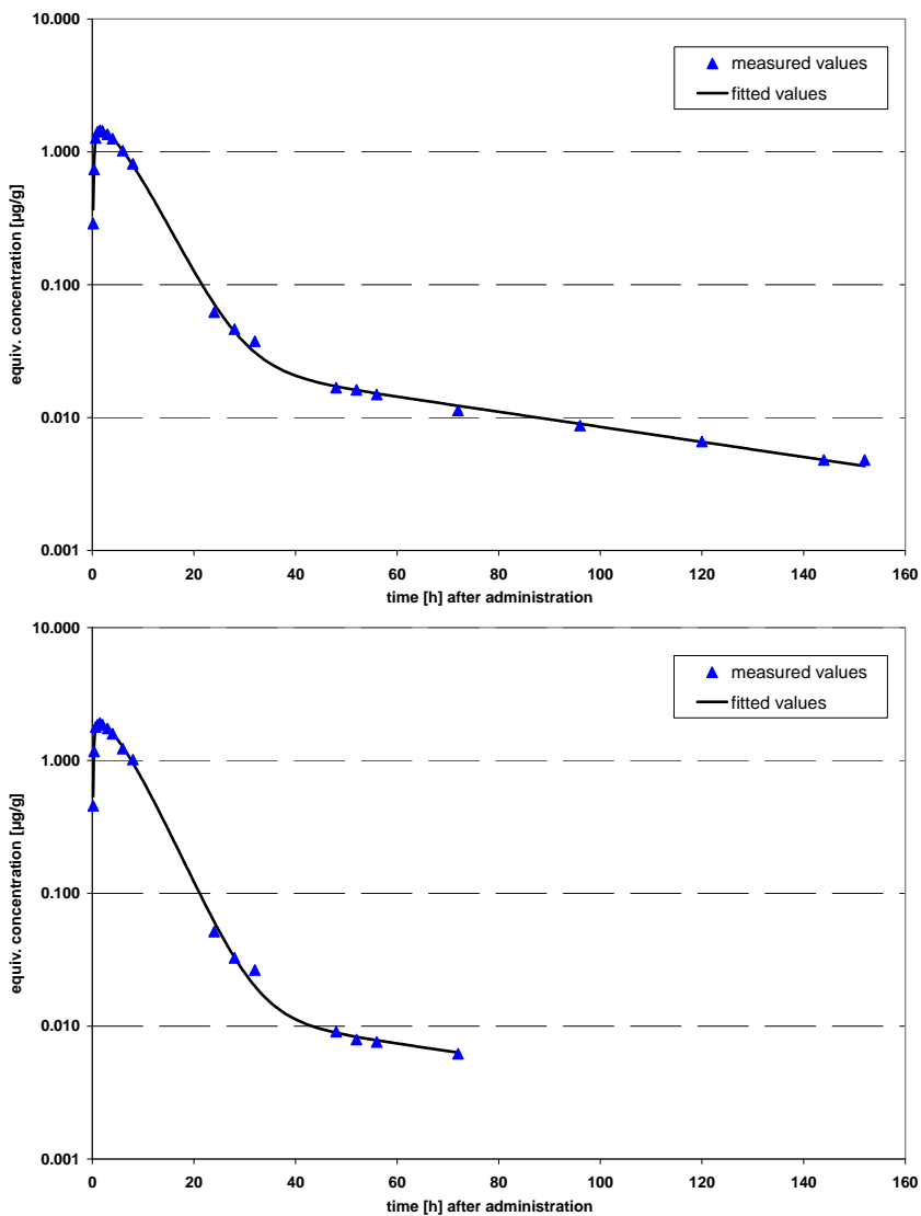
Figure 2: Timecourse of radioactivity in the plasma following a single oral dose of [furanone-4- 14 C] flupyradifurone (2 mg/kg bw). (upper curve: male rats; lower curve: female rats)
