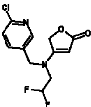
Figure 6: Chemical structure of BYI 02960 (flupyradifurone).
