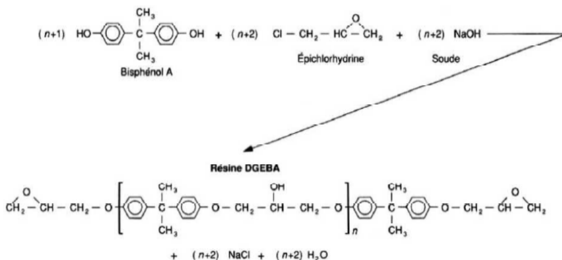
Figure 2 : Synthesis of resins based on bisphenol A (ANSES, 2011)
