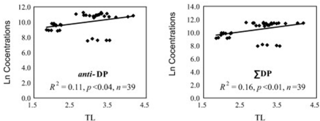
Figure 5: Regressions between trophic level and concentrations of Dechlorane Plus (anti- and total isomers) in aquatic species
