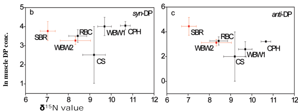
Figure 3: Relationship between \delta^{15}\text{N} and Dechlorane Plus muscle concentrations in wild birds from South China
