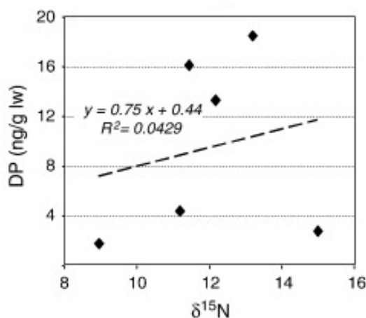
Figure 6: Plot of mean total Dechlorane Plus concentrations in falconiform eggs versus \delta^{15}\text{N}
