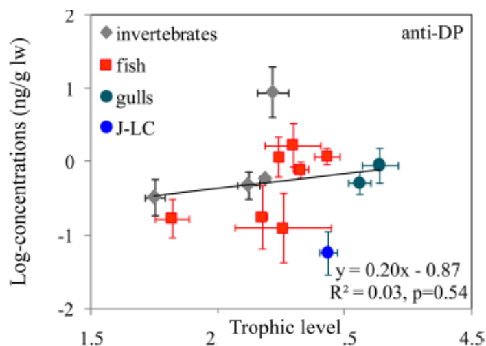
Figure 4: Regressions between trophic level and concentrations of anti-Dechlorane Plus in aquatic species in a Chinese marine food web (error bars represent \pm 1 standard error)
