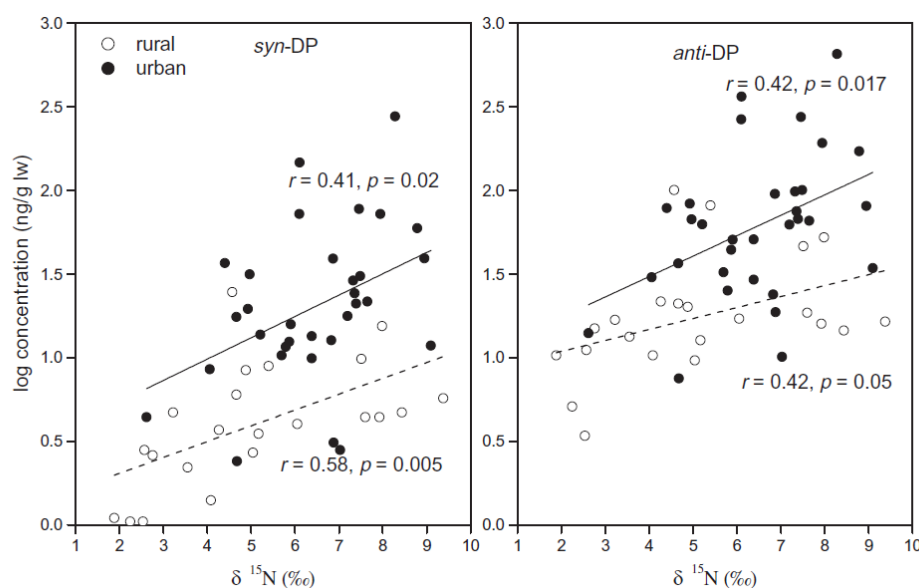
Figure 7: Plot of mean Dechlorane Plus concentrations in passerine muscle versus \delta^{15}\text{N}
